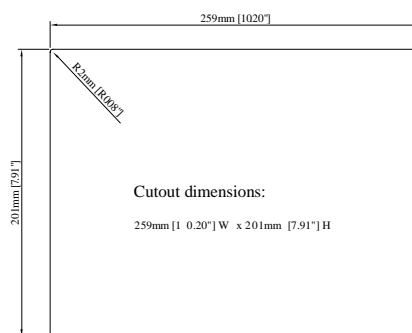
Panel Cutout
