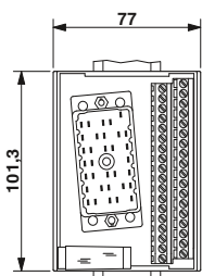
Чертеж UMK-EC90/32/EX-XOL
