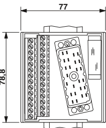
Чертеж UMK-EC56/25/EX-R
