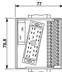
Чертеж UMK-EC56/25/EX-L
