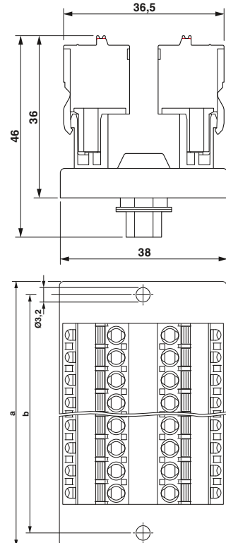
Чертеж DFLK-D...SUB...FKCT
